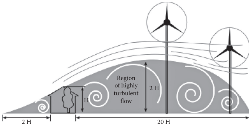
FIGURE 9.2 Height of small wind turbine near obstacles of height H .
