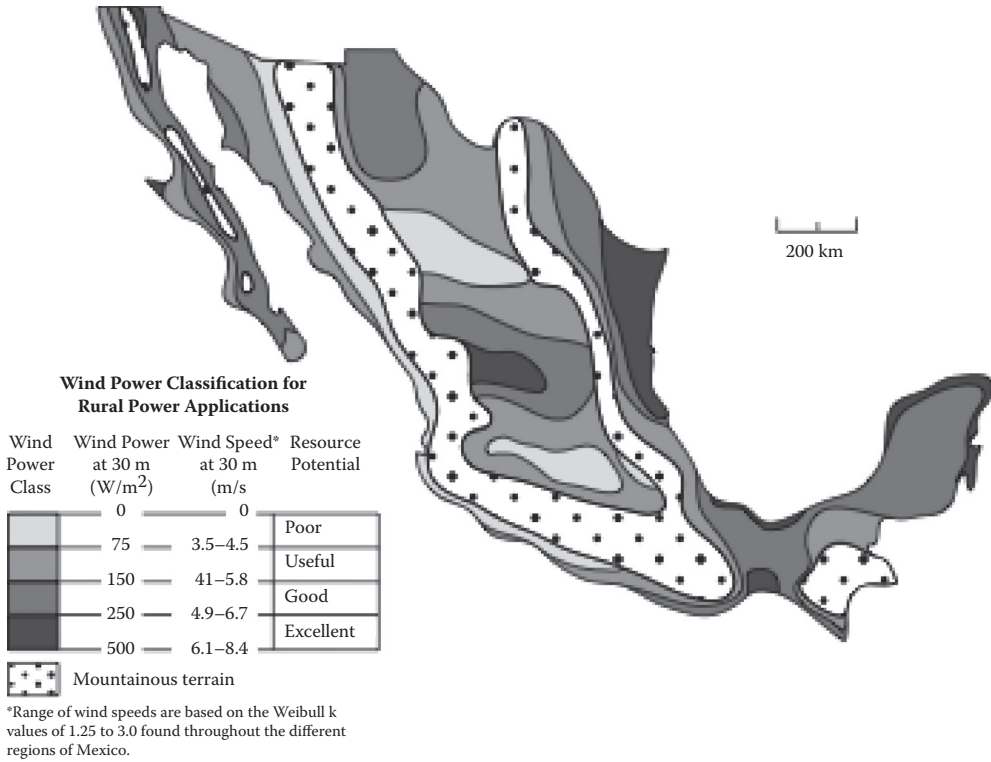
FIGURE 9.1 Wind power map for rural applications In Mexico. Notice difference in definition of wind power class and height at 30 m.
