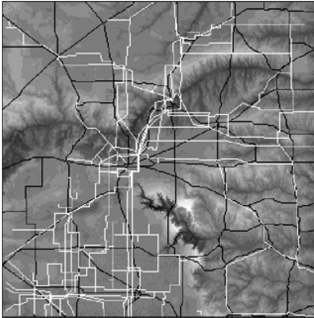
FIGURE 9.8 Terrain exposure from the average elevation for Texas Panhandle showing major highways and transmission lines. Light areas have better exposure (range of 16 levels from -195 m to +168 m height).
