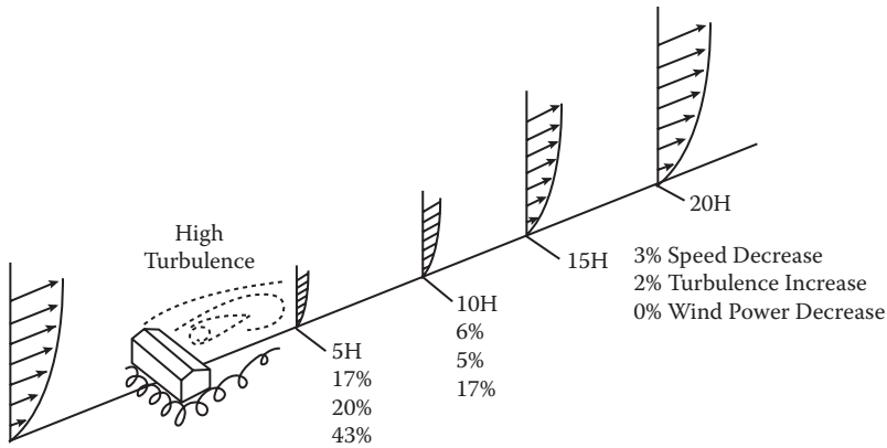
FIGURE 9.3 Estimate of speed, power decrease, and turbulence increase for flow over building. Estimates shown are for building height H . (Source: M.N. Schwartz and D.L. Elliott. 1995. In Proceedings of Windpower Conference . With permission.)
